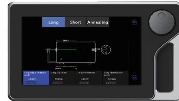
Mode Selection
